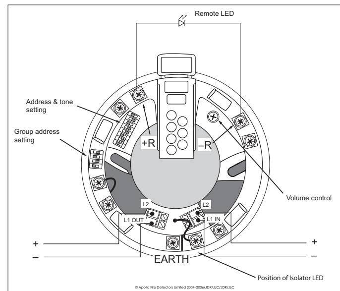
Fig. 1 Sounder VAD Base with isolator wiring
