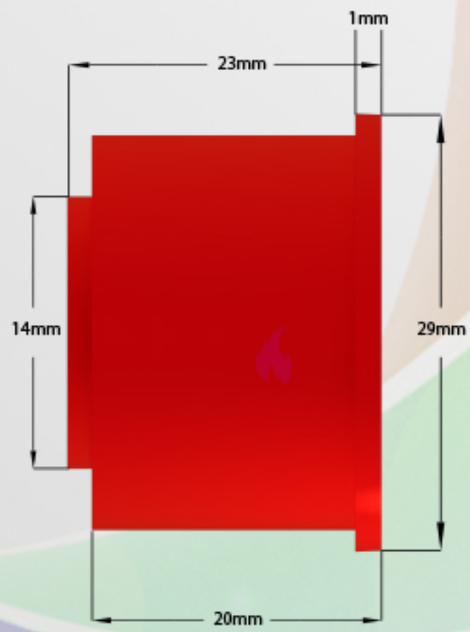
Capillary Adaptor
