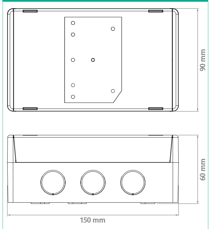
Figure 1: Intelligent Twin Switch Monitor dimensional drawing
