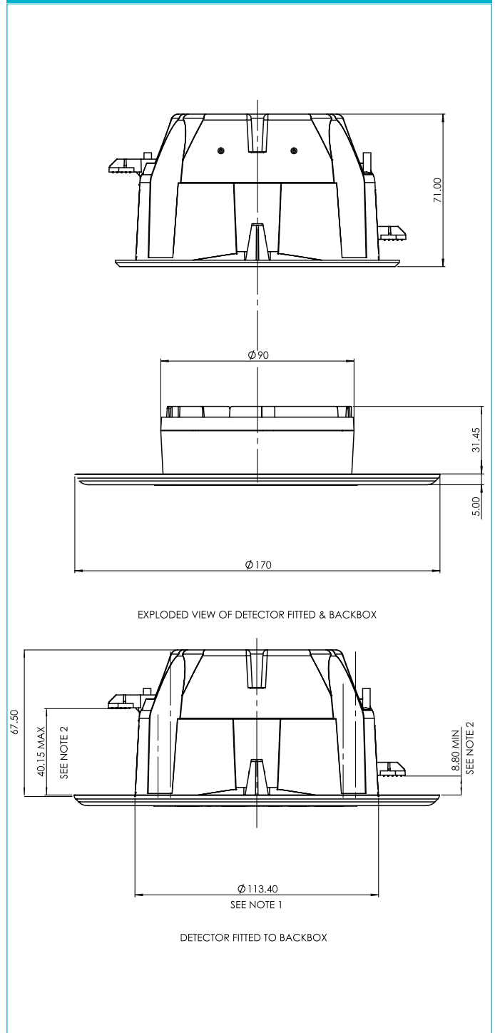
Figure 1: Soteria Dimension Specialist Optical Detector dimensional drawing
